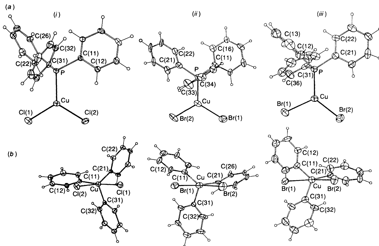
Fig. 1 The [\text{Cu}(\text{PPh}_3)\text{X}_2]^- anions projected (a) normal to the \text{PCuX}_2 plane, and (b) down \text{Cu-P} ; (i)–(iii) \text{X} = \text{Cl} or \text{Br} ( \text{NPr}_4 or \text{NBu}_4 ). 20% Thermal ellipsoids are shown for the non-hydrogen atoms; hydrogen atoms have arbitrary radii of 0.1 Å
